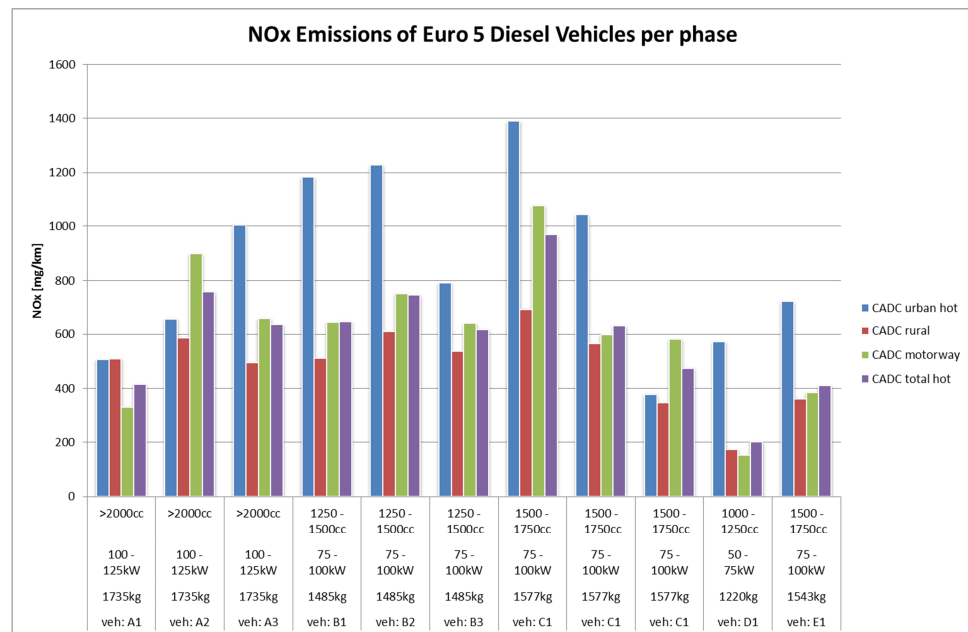
Figure 2: The CADC as real-world emission. The test result of the 11 vehicles tested, separate of each part: urban, rural, and motorway (130 km/h), and combined.
